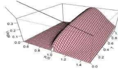
Mean Reversal Strategy
